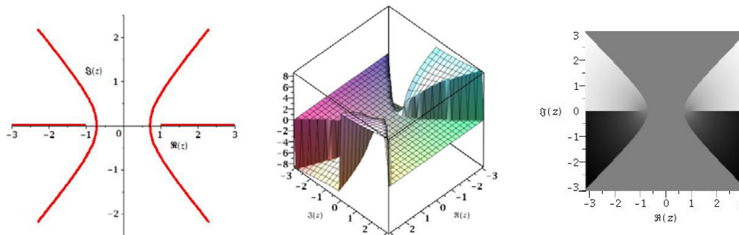
Figure 2: Visualising the branch cuts of equation (4).
